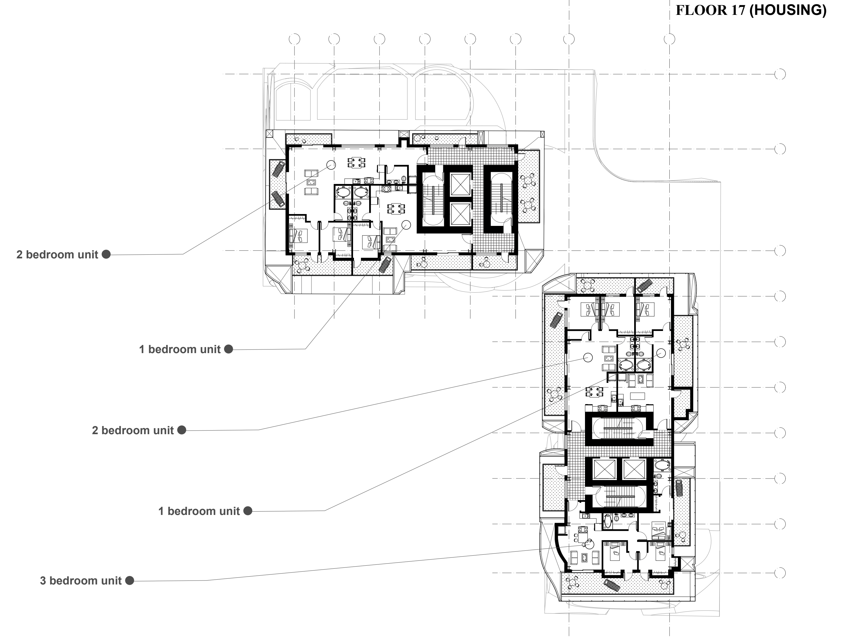
FLOOR 17 (HOUSING)
